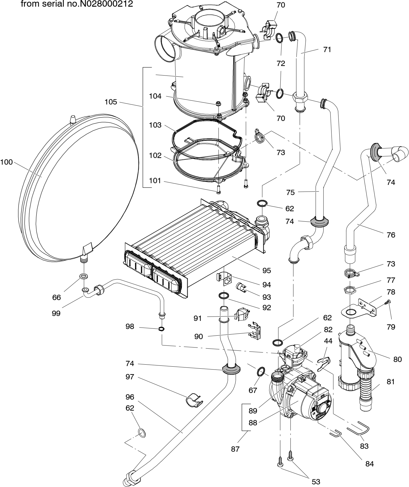
Pump and main circuit assembly from serial no.N028000212
